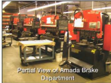
Amada Promecam HFB1003 CNC Press Brake
