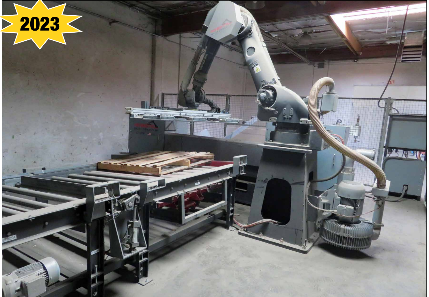
Alliance Robotic Pallet Dismantler w/Yaskawa Motomen HP3 Robotic Arm
