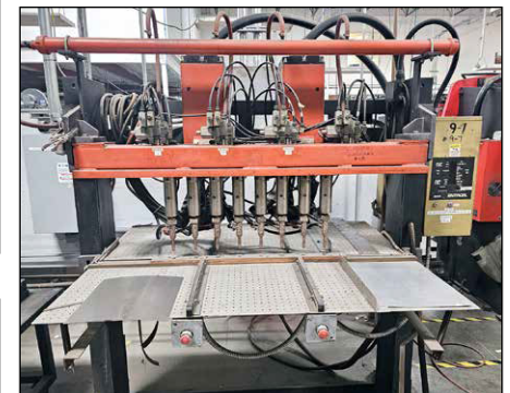
Janda M6081201C2T, 120 KVA Multi Head Spot Welder
