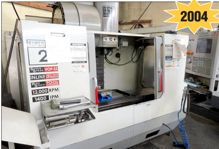
2004 Haas Super VF2, 12,000 RPM CNC Vertical Machine Center
