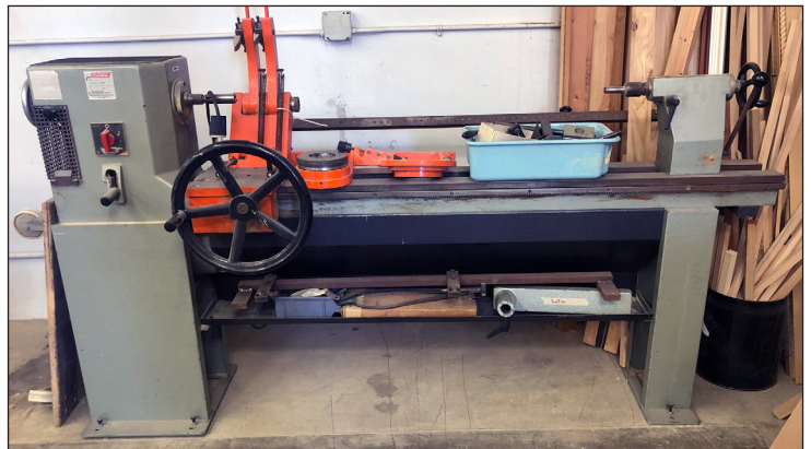
Hapfo Type AP 5000-M Wood Lathe
