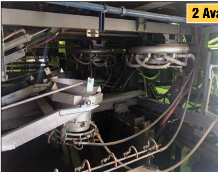
Custom Built Glass Fiberizers
