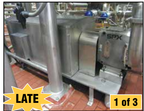
SPX Homogenizer
