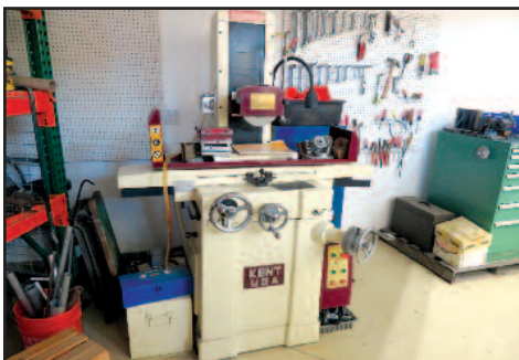
Kent Mdl. KGS618, 6" x 18" Manual Surface Grinder
