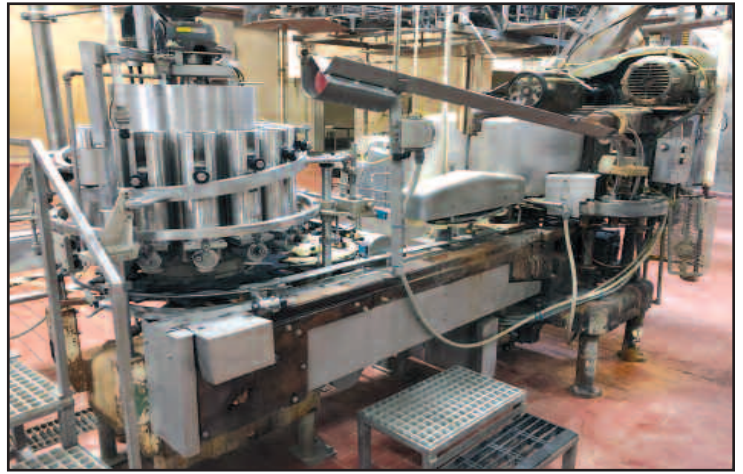
Angleus Mdl. 60L 6-Head Can Seamer
