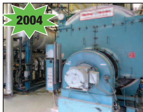
Cleaver Brooks Mdl. CEW-700-600-150, 600hp Boiler
