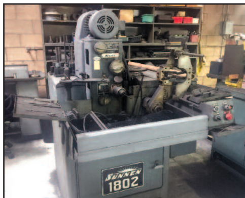
Sunnen Mod. MBC-1802 Precision Horizontal Hone
