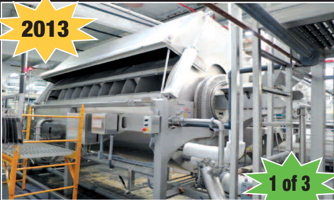
Lyco 8600, 6' Dia. X 12' Vapor Flow Blancher
