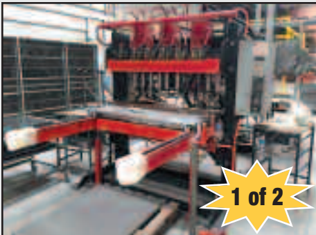
Janda 120 KVA Multi Head Spot Welders
