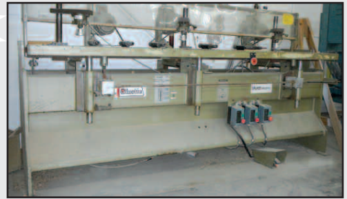
Doucet Sicotte Mod. 750-8 Horizontal Boring Machine
