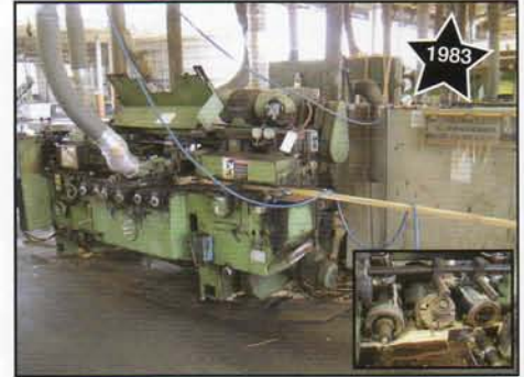
Weinig U22A, 6-Spindle Moulder (inset: Tilting Second Right On Weinig U22A)
