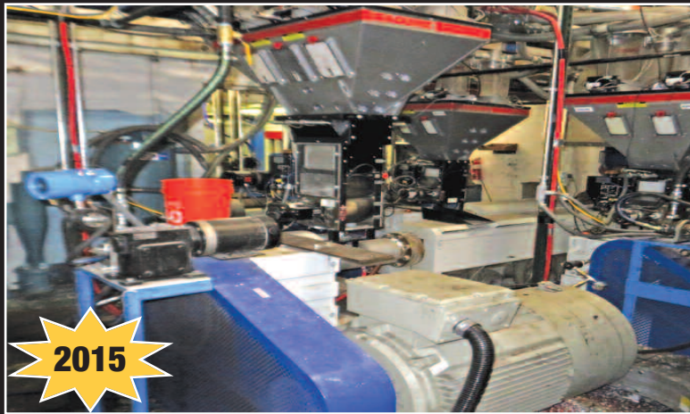
Lung Meng RCT 55-90-55, 3-Layer Blown Film Line
