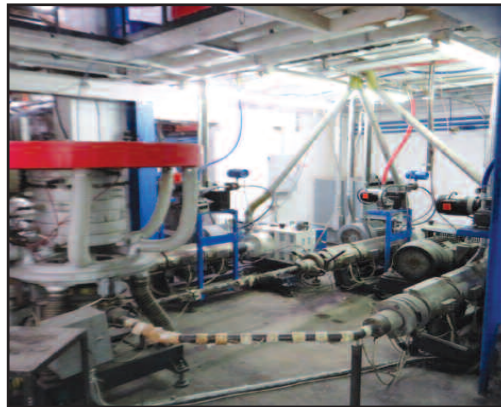
3-Layer Blown Film Line
