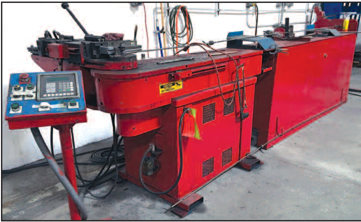
Bantec Mod. BT-220, 2" Horizontal Tube Bender
