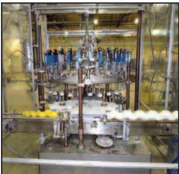
Pneumatic Scale 32HD Rotary Filler
