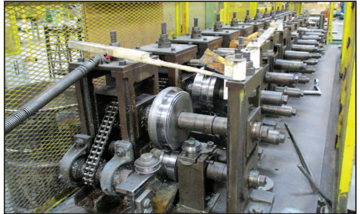
4" x 12 Stand 1-1/2" Arbors w/Payoff Reel & Chop Saw
